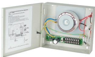
PW408S 4A/8port DC12V/AC24V
